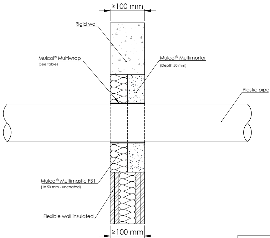
Drawing: FW.E-PP-MW2-MM2.5.10
