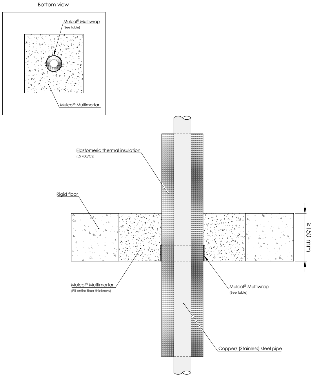
Drawing: RF.E-CU-MW-MM1.3.22
