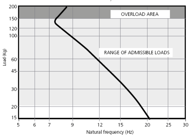
CUSHIONING FREQUENCY Vibrafon CHP HD 150
