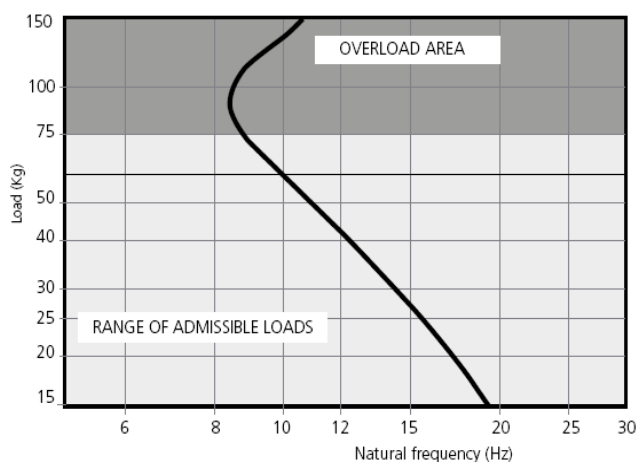
CUSHIONING FREQUENCY Vibrafon CHP 75
