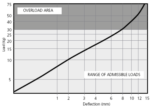
DEFLECTION DIAGRAM Vibrafon CHP 30
