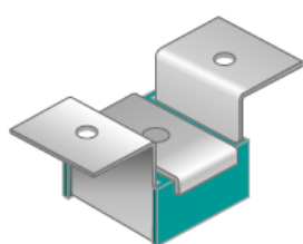
VibraFon CHP 1 Direct mounting on the ceiling by means of 2 screws
