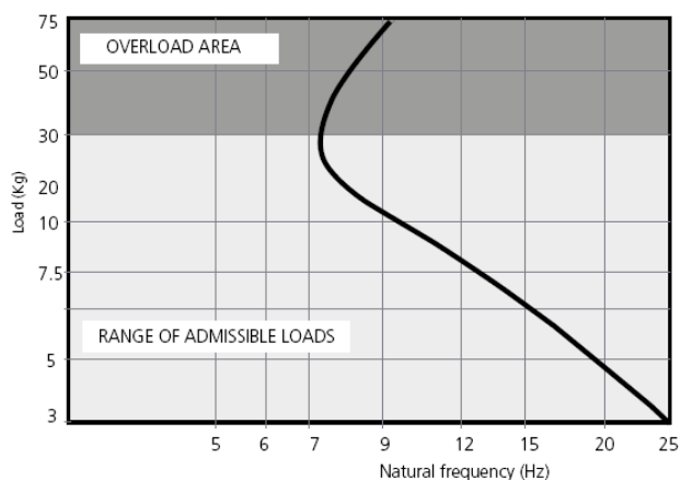
CUSHIONING FREQUENCY Vibrafon CHP 30
