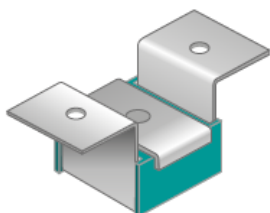
VibraFon CHP HD 1 Direct mounting on the ceiling by means of 2 screws
