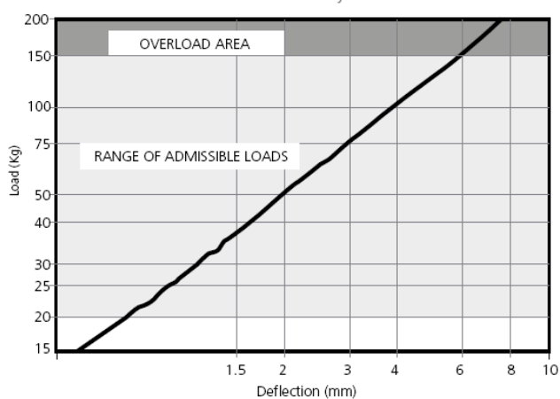
DEFLECTION DIAGRAM Vibrafon CHP HD 150
