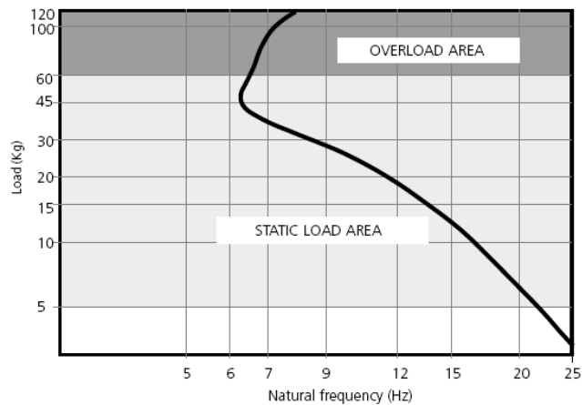
CUSHIONING FREQUENCY Vibrafon CHP HD 150
