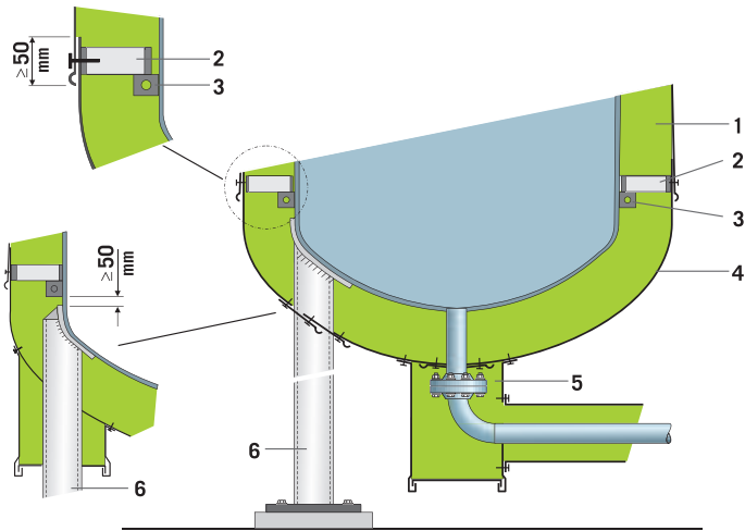
1. Insulation: e.g. ProRox Wired Mats - 2. Support construction - 3. Mounting support - 4. Conical column head - 5. Vessel outlet - 6. Vessel leg
