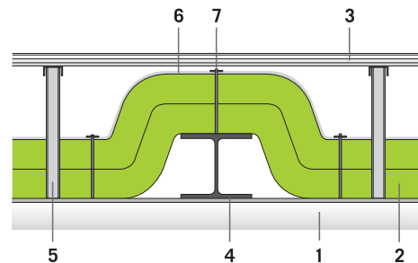
1. Duct wall - 2. Insulation: ProRox Wired Mats - 3. Metal cladding: corrugated sheet - 4. Reinforcing element - 5. Supporting construction and spacer - 6. Aluminium foil (optional) - 7. Welding pins/clips
