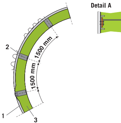
1. Tank wall - 2. Spacer - 3. Insulation: e.g. ProRox SL 930 semi rigid slab
