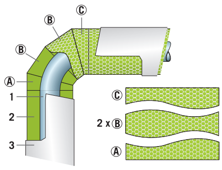
1. Pipe - 2. ProRox Insulation - 3. Cladding - A to C: Elbow segments of mats
