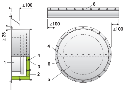
1. Manhole - 2. Insulation: e.g. ProRox MA 520 ALU load bearing mats - 3. Cladding - 4. Sheet-metal screw (Self tappers or blind rivets) - 5. Cladding - 6. Sheet metal screw (self-tappers)
