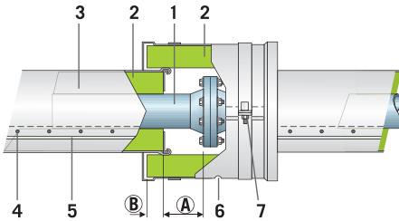
1. Pipe - 2. Insulation: e.g. ProRox Wired Mats - 3. Cladding - 4. Sheet-metal screw or rivet - 5. Swage - 6. Drainage opening - 7. Straps - \textcircled{B} \geq 50 \text{ mm} - \textcircled{A} = \text{Bolt length} + 30 \text{ mm}
