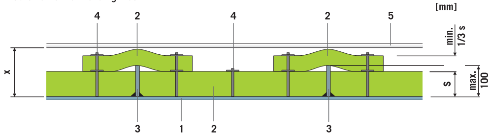
1. Duct wall - 2. Insulation: ProRox Wired Mats - 3. Reinforcing ribs - 4. Welding pins with clips - 5. Metal cladding
