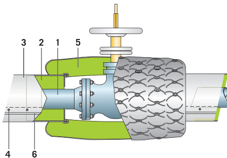
1. Pipe - 2. Insulation: e.g. ProRox Pipe Sections - 3. Cladding - 4. Sheet-metal screw or rivet - 5. Removable coverings (insulated from the inside with e.g. ProRox Wired Mats) - 6. Swage
