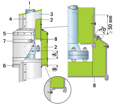
1. Pipe - 2. Insulation: ProRox Wired Mats - 3. Sheet - 4. Sheet-metal screw or rivet - 5. Rain deflector - 6. Lock washer - 7. Straps - 8. Lock washer - \textcircled{B} \geq 50 \text{ mm} - \textcircled{A} = \text{Screw length} + 30 \text{ mm}
