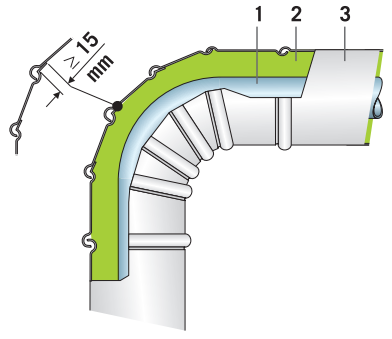
1. Pipe - 2. ProRox Insulation - 3. Cladding
