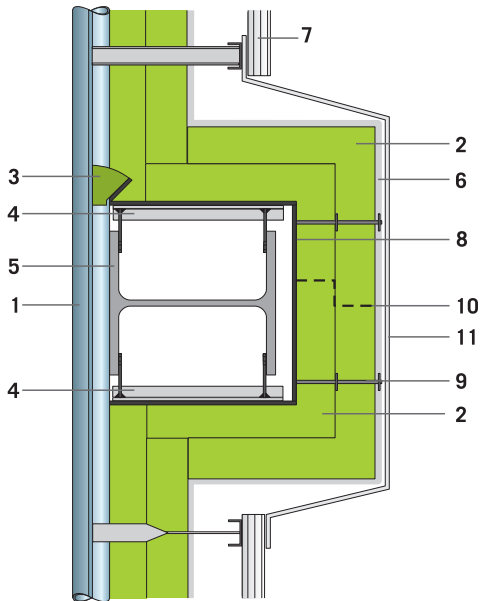
Buckstays exposed to heat on a boiler wall
