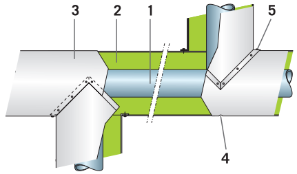
1. Pipe - 2. ProRox Insulation - 3. Cladding - 4. Drainage opening - 5. Edging with mastic compound
