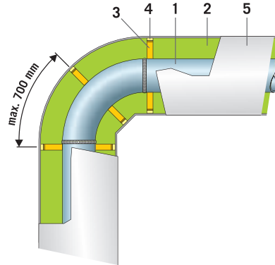
The spacers on pipes are located under the 1. Pipe - 2. ProRox Insulation - 3. Spacer - 4. Thermal dividing layer - 5. Cladding
