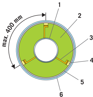
1. Pipe - 2. ProRox Insulation - 3. Spacer - 4. Thermal dividing layer - 5. Support ring - 6. Cladding
