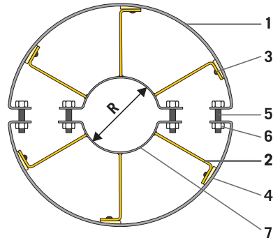
1. Support ring - 2. Bar - 3. Rivet or screw connection - 4. Thermal decoupling - 5. Clamping screw - 6. Screw nut - 7. Internal clamping ring
