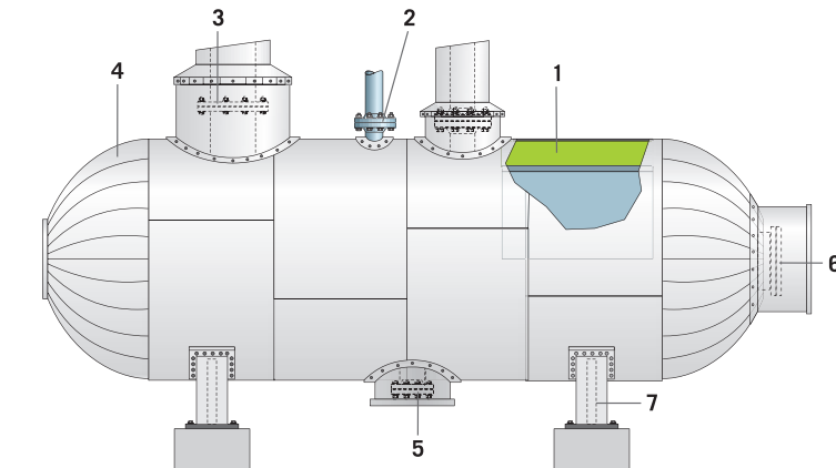
1. Insulation: ProRox load bearings Mats - 2. Flange inlet for safety valve - 3. Vessel filling nozzles - 4. Conical head - 5. Vessel drawdown - 6. Conical head with manhole - 7. Vessel leg
