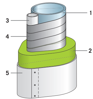
1. Pipe - 2. Insulation: ProRox load bearing Mats or Wired Mats - 3. Tracing - 4. Aluminium foil - 5. Cladding
