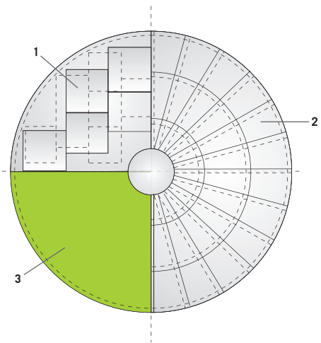
1. Finishing with aluminium cladding - 2. Finishing with steel radial segments - 3. Insulation: ProRox SL Slabs
