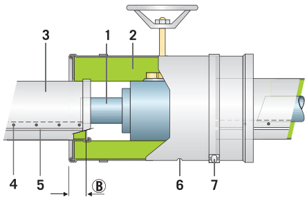
1. Pipe - 2. Insulation: ProRox Wired Mats - 3. Cladding - 4. Sheet-metal screw or rivet - 5. Swage - 6. Drainage opening - 7. Straps - \textcircled{B} \geq 50 \text{ mm}
